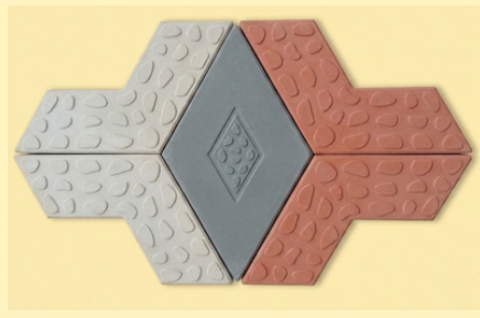
V & KISU COMBO PAVINGS Thickness: 4Cm 52 Pcs/SQM OffWhite, Red & Grey
