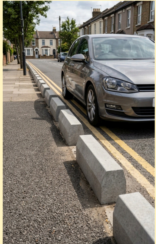
HEAVY DUTY KERBSTONE SIZE: 50x35 Cm THICKNESS: 15Cm COLOR: GREY.
