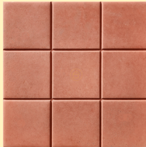
DRAFT 9 FLOOR TILES 30x30Cm > 11 Pcs/SQM Thickness: 2 Cm OffWhite, Red & Grey
